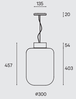
S suspended
